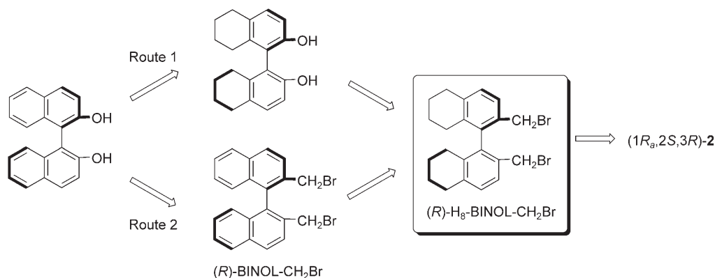
Scheme 1. Synthetic analysis of (1 R a ,2 S ,3 R )-2.
