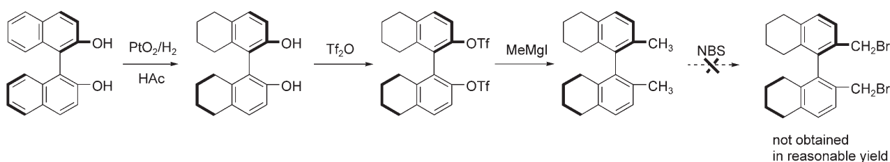
Scheme 2. Synthetic approach from ( R )-H 8 -BINOL.
