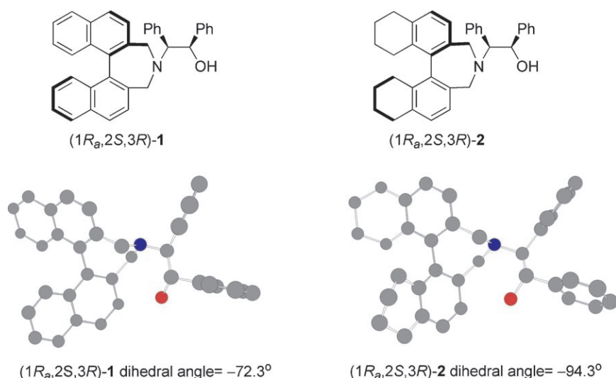
Figure 1. Molecular structures of (1 R a ,2 S ,3 R )-1 and (1 R a ,2 S ,3 R )-2. The hydrogen atoms are omitted for the purpose of clarity. The dihedral angles of the axial biaryl groups were estimated by ChemDraw 3D calculations (MM2). (The minus sign is arbitrarily given by the program.)
