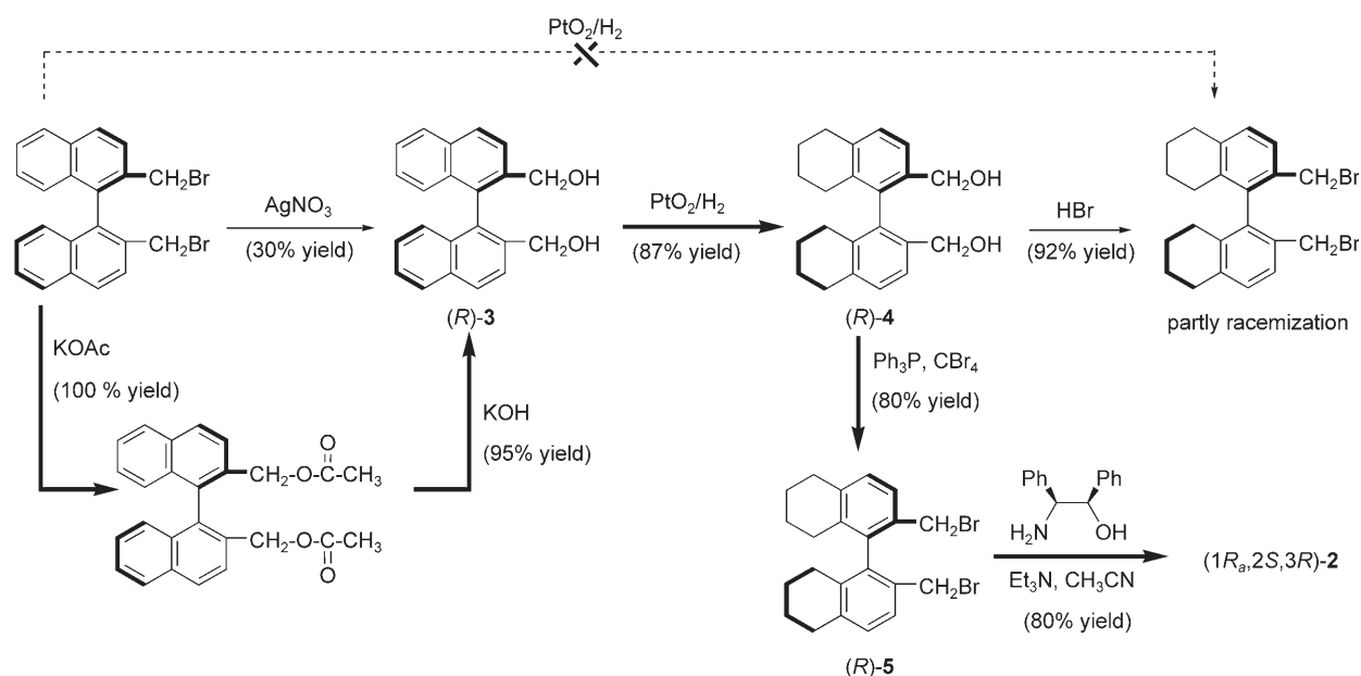
Scheme 3. Synthetic approach from (R)-BINOL-CH 2 Br.
