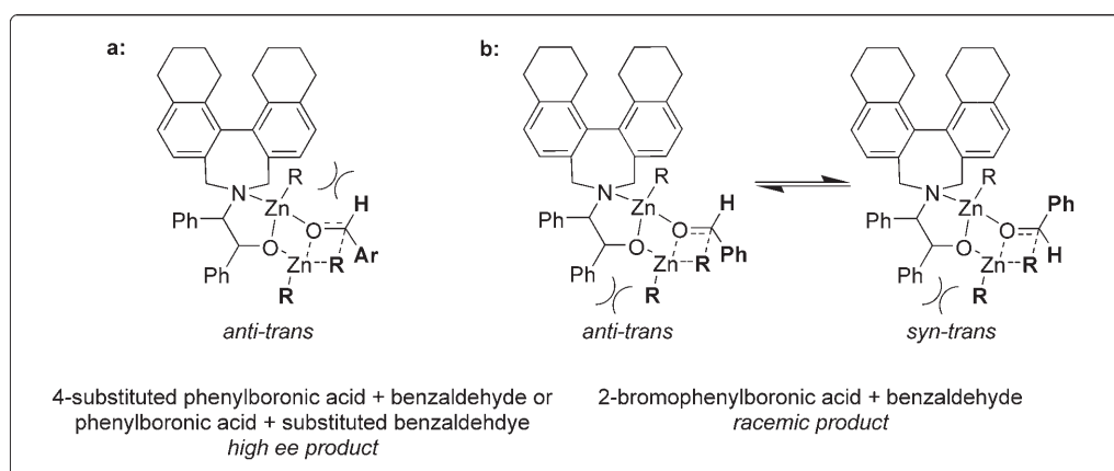
Figure 2. Proposed transition states for the asymmetric arylation of aldehydes.
